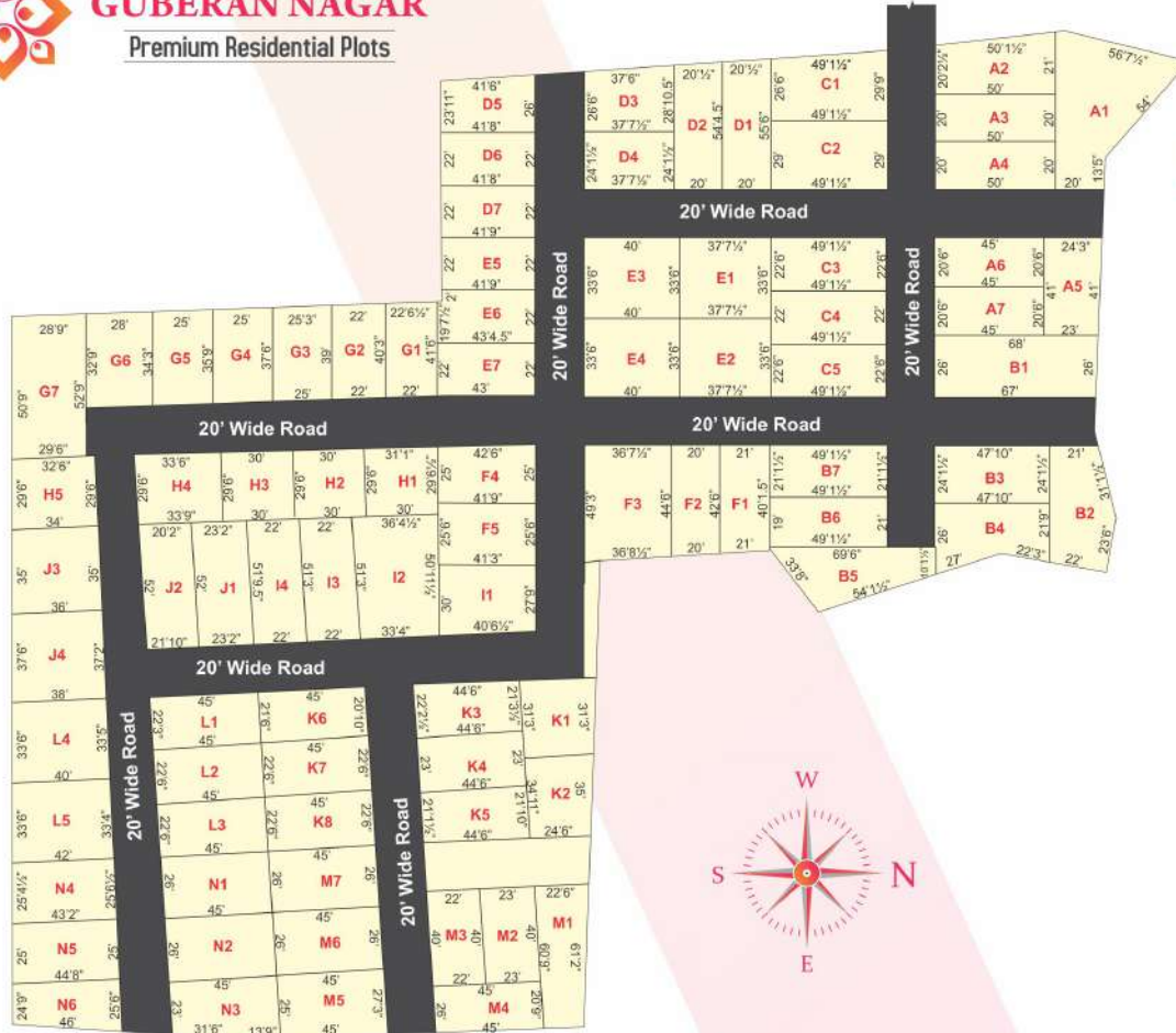
Plan Showing the Proposed Sub Division of House Sites in S.No: 394/1A, 1B, 2A, 2B, 2C, 2D at Paruthipattu Village, Poonamalle Taluk, Thiruvallur (Dt)
